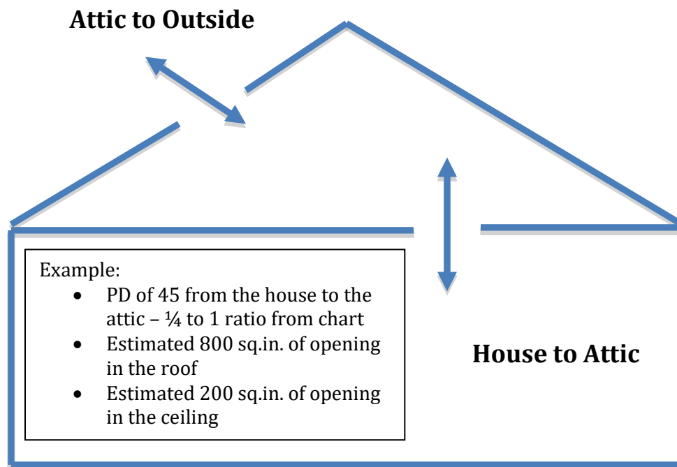
Zone Pressures
